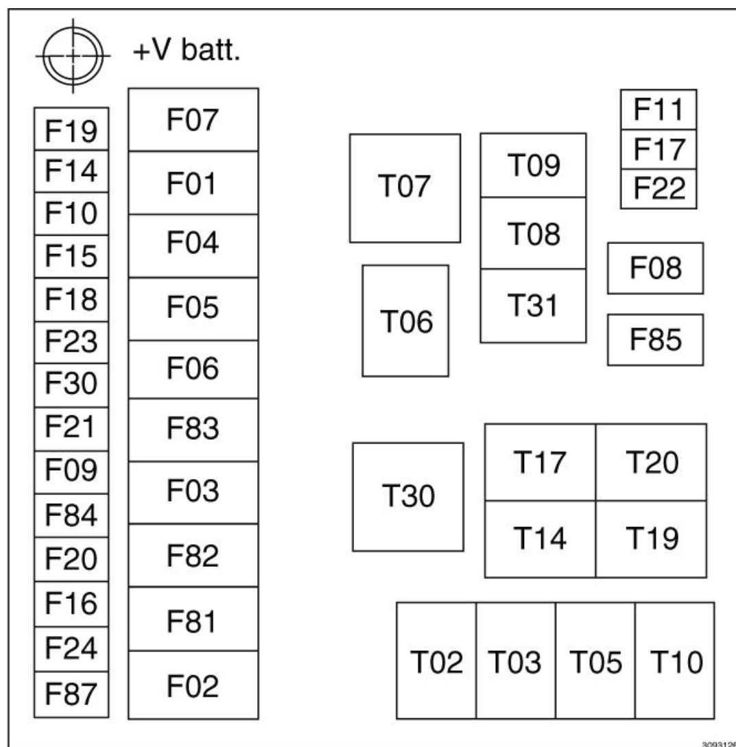
Fig. 6: Second Fuse Panel
